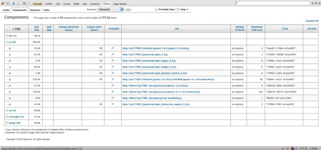
Figure 1-12. Components view in YSlow
