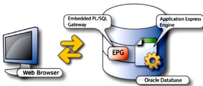
Figure 1-2. Using the Embedded PL/SQL Gateway
